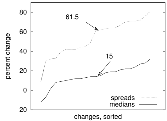
Figure 8: Range of changes in median and spread generated by applying the recommendations of either \mathcal{W} or SEESAW. The median observed changes were (15, 61.5)% for (medians, spreads), respectively. For the sake of brevity, this graph ignores the -119% outlier value seen in OSP2 defects.
