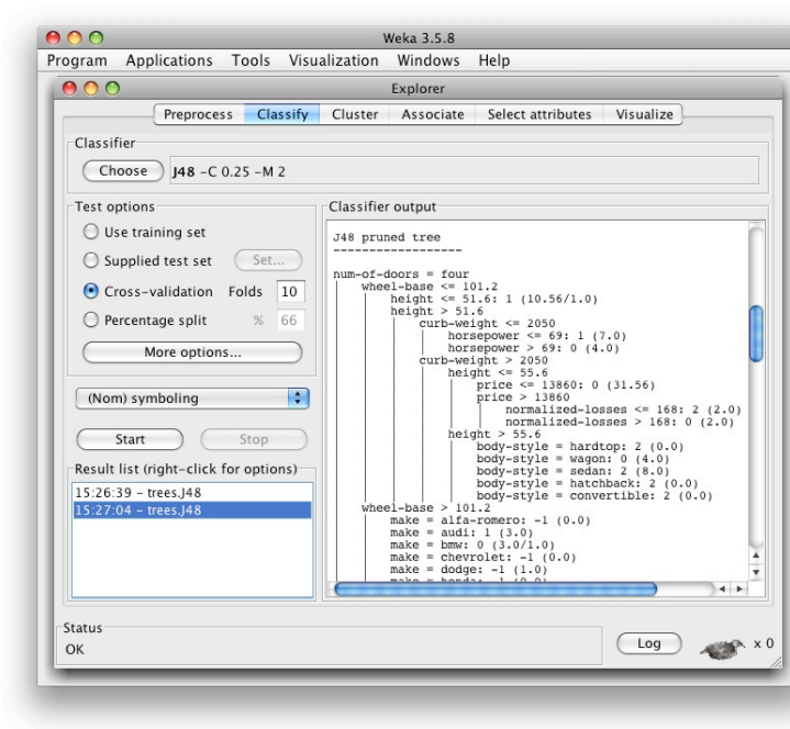
Figure 1. The WEKA toolit running the J48 decision tree learner.
