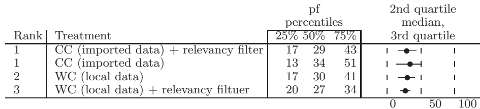
Figure 16. Probability of False Alarm (PF) results, sorted by median values.
