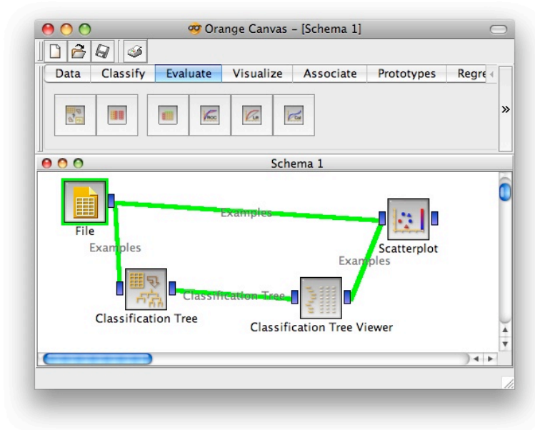
Figure 2. Orange’s visual programming environment. Green lines indicate data streams passed between functions.
