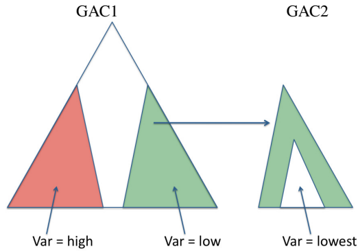
Figure 4: Execution of TEAK on 2 GAC trees, where tree on the left is GAC1 and the one on the right is GAC2 (i.e. lower variance sub-tree of GAC1). The instances in the low variance region of GAC1 (green region) are selected to form GAC2. Then test instance traverses GAC2 until no decrease in effort variance is possible. Wherever the test instance stops is retrieved as the subtree to be used for adaptation (white region of GAC2).
